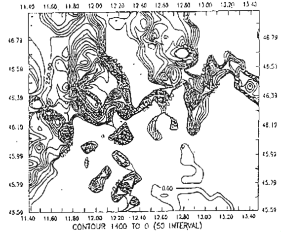
RESIDUAL MAGNETIC OF PAZUNDAUNG CHAUNG
