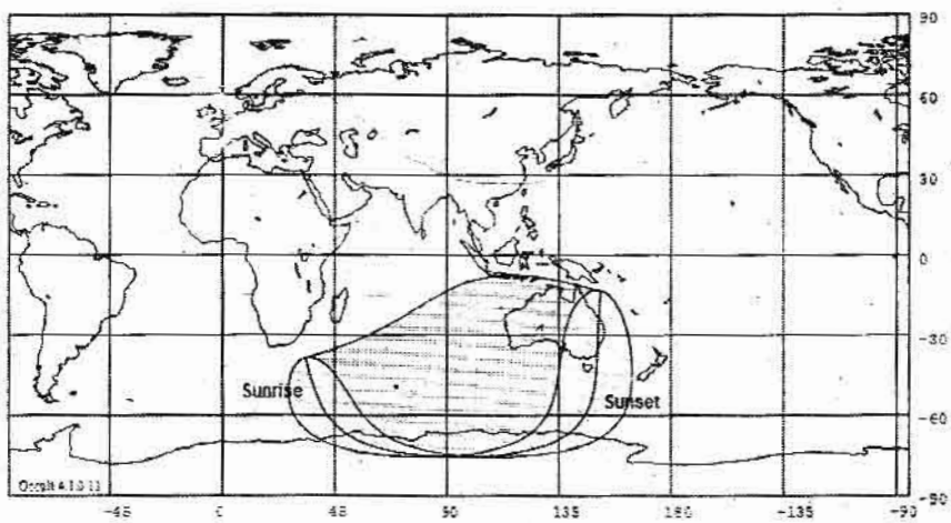
In PALE BLUE region of partial eclipse, YELLOW sun rises or sets in eclipse
