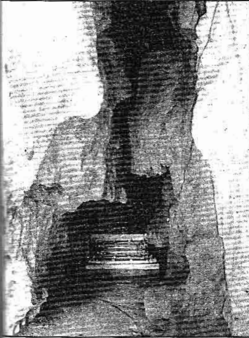
Ancient caves, such as 'Nat Pya cave' & 'Lin Noe (Bat) cave' are situated near 'Kaung Hkar' village and 'Nam Hkite' village in 'Mae Han' village tract in Lashio Township. Nat Pya cave is situated in the eastern part of Kaung Hkar village & Lin Noe cave is situated near Nam Hkite village.
