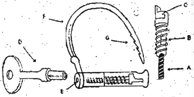
1. Threaded portion of Bolt. B. Spring. C. Part of Bolt that engages notches on Stock. D. Key. E. Key-hole. F. Handle. G. Notches on Stock.
