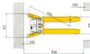
SDJ series with fixed forks
