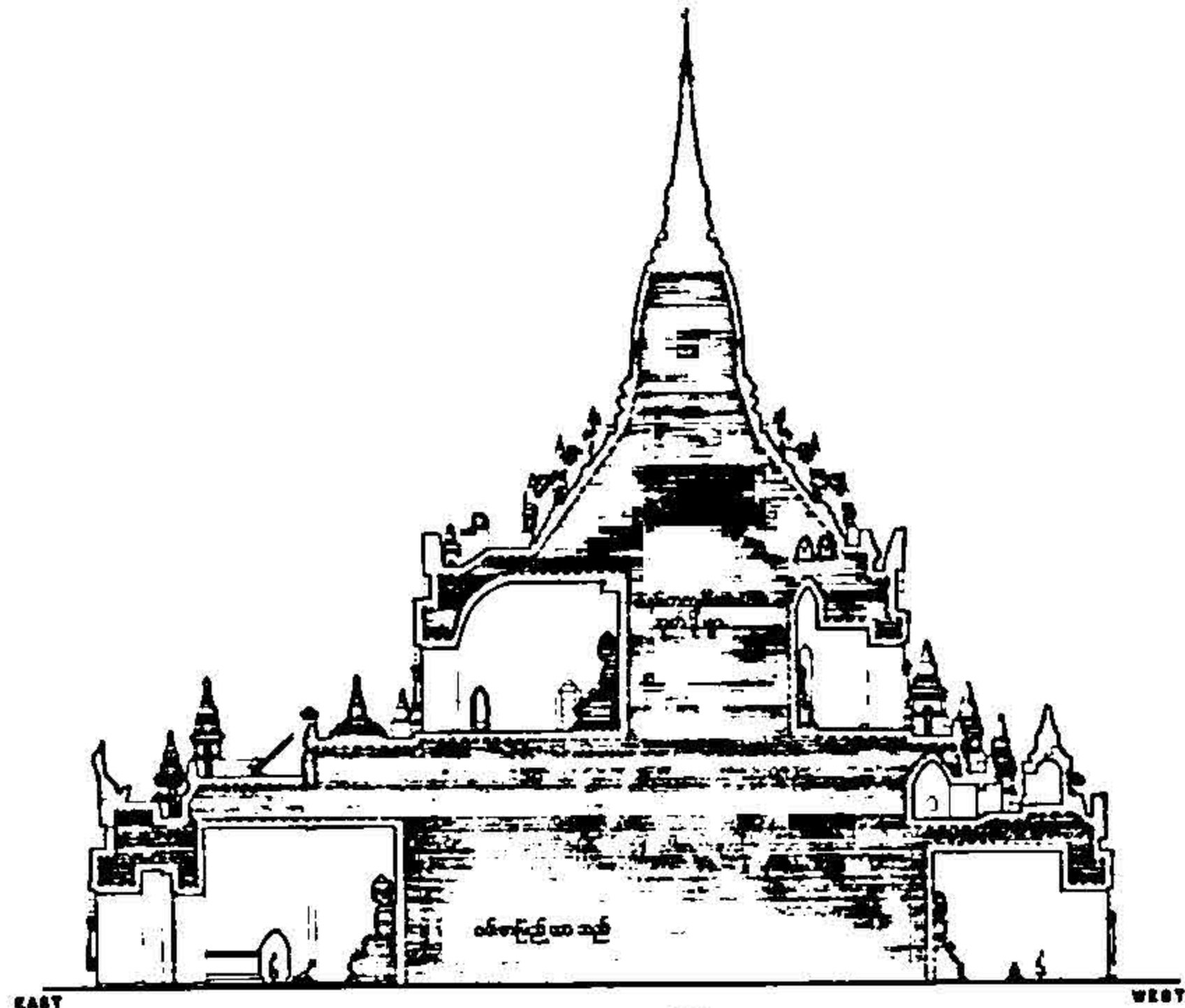
GAWDAWPALIN. BUILT BY NARAPATISITHU 1175 - 1210 A.D. SECTION THROUGH EAST WEST. DEPARTMENT OF ARCHITECTURE RABSOON INSTITUTE OF TECHNOLOGY
