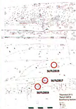
SMT stratigraphy with OSL dating locations
