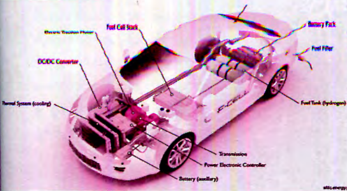
Hydrogen Fuel Cell Electric Vehicle
